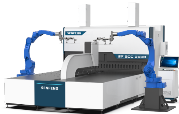
Robot-assisted Panel Bender
